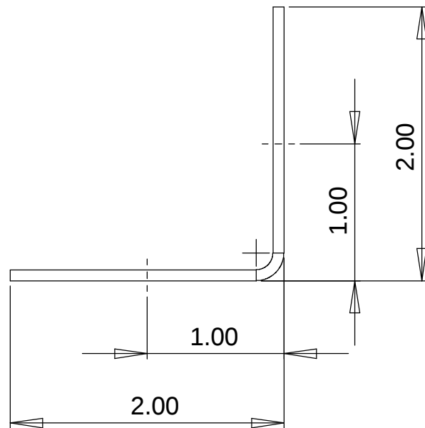
Side View [1:1]
